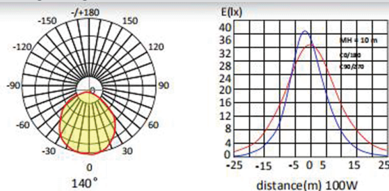
Lighting Distribution and Illumination curve
