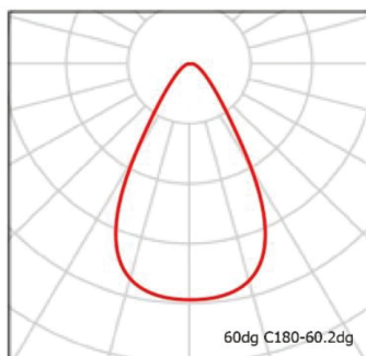
Lighting Distribution Curve
